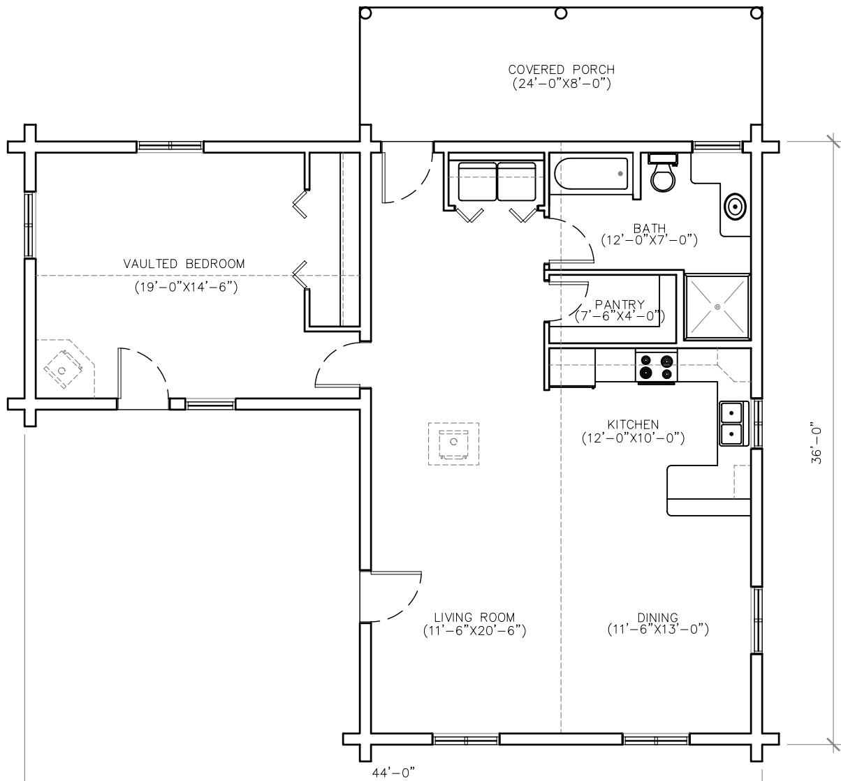
FLOOR PLAN
