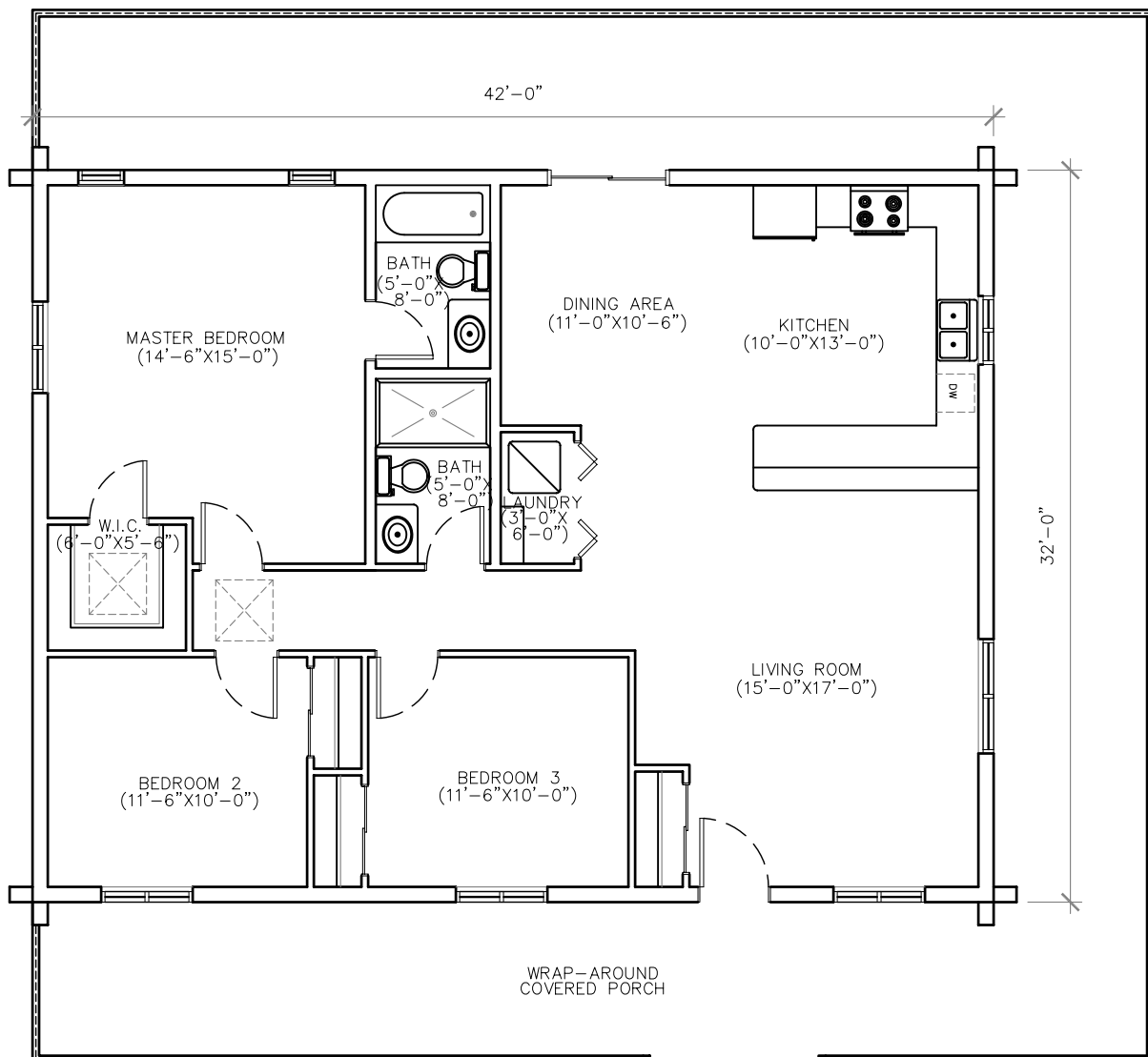
FLOOR PLAN
