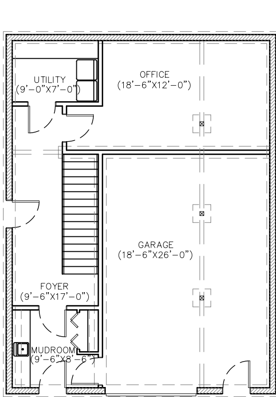
BASEMENT/GARAGE PLAN
